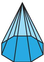
Octagonal pyramid
