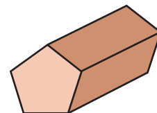
Pentagonal prism
