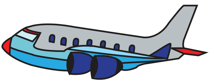
AIRPLANE
